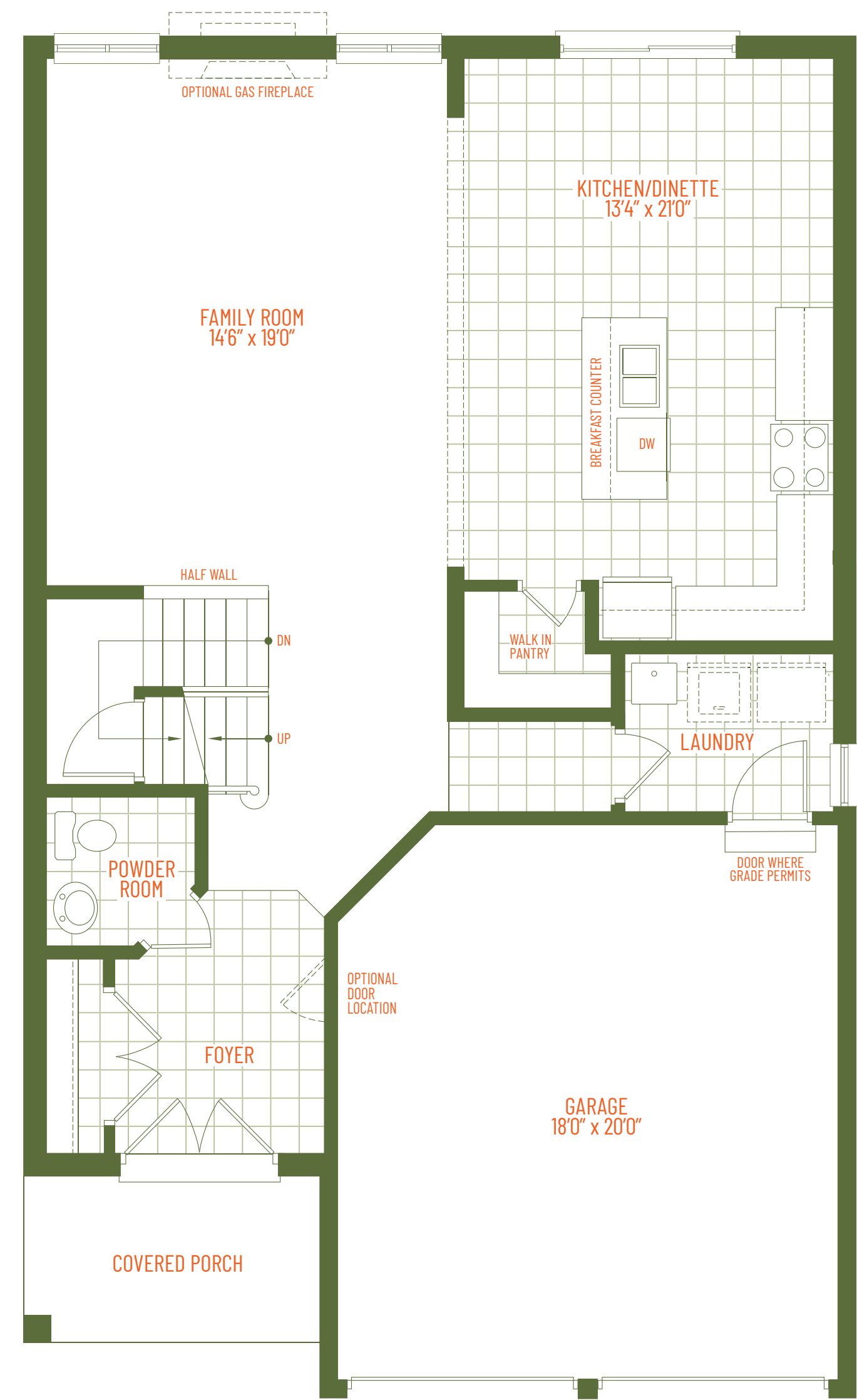
MAIN FLOOR PLAN ELEVATION A & B
