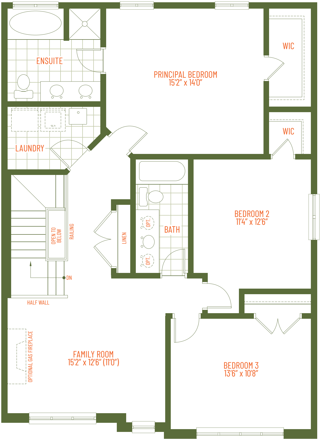
SECOND FLOOR PLAN ELEVATION A
