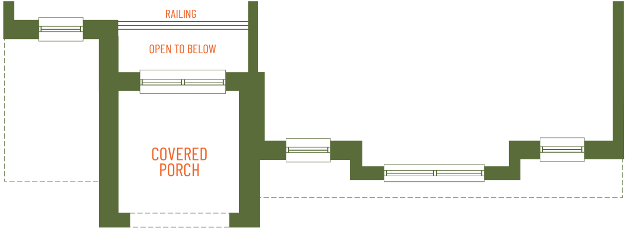
SECOND FLOOR PLAN ELEVATION C
