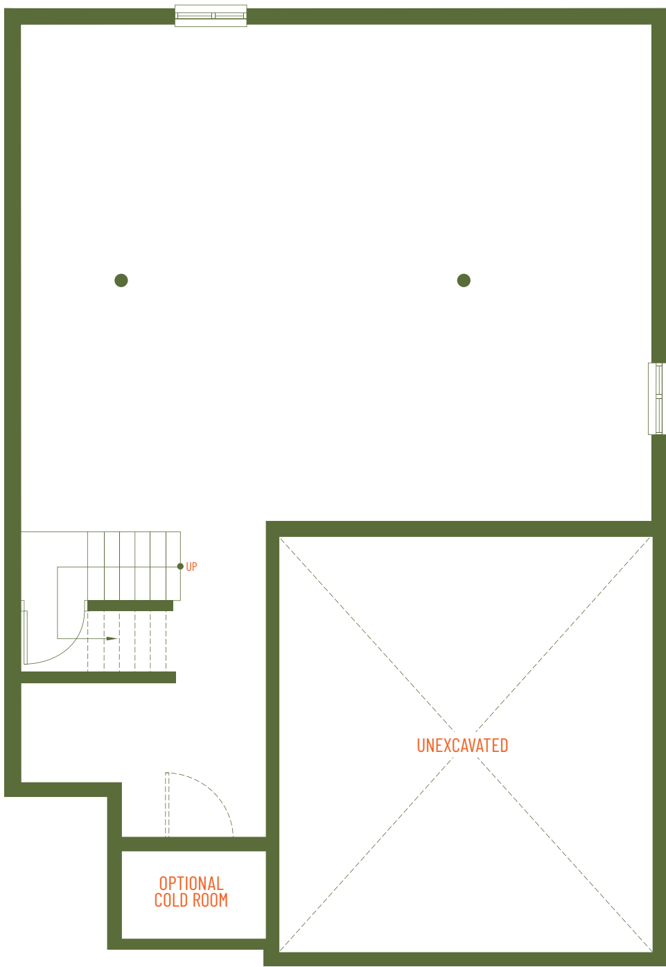
BASEMENT FLOOR PLAN ELEVATION A
