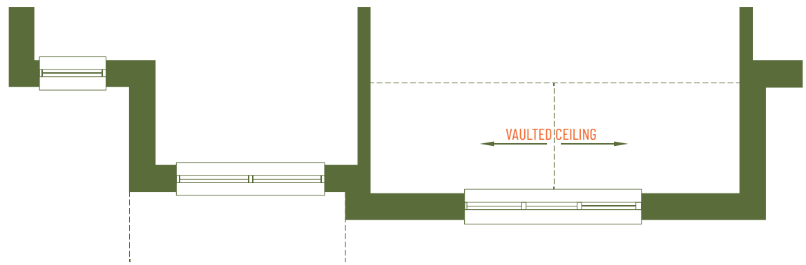
SECOND FLOOR PLAN ELEVATION B
