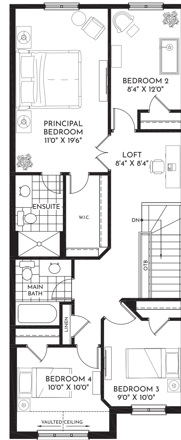
OPT. SECOND FLOOR - 4 BEDROOM
