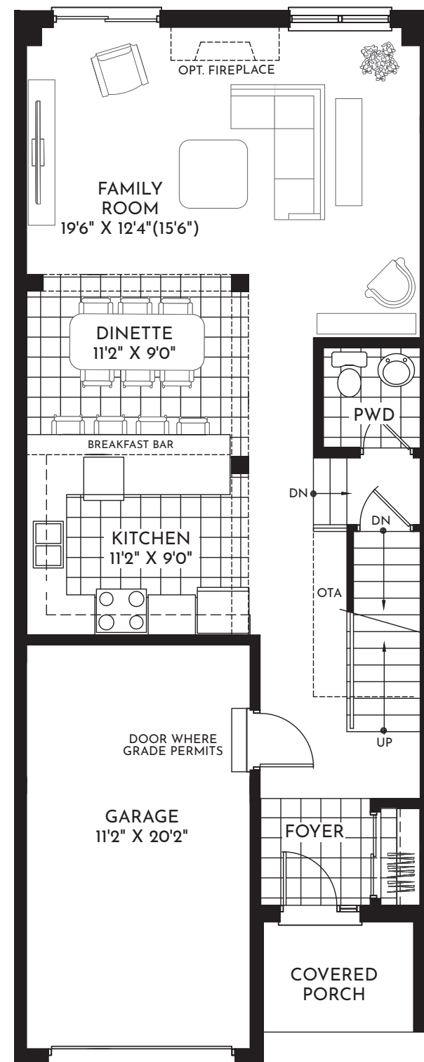
MAIN FLOOR
