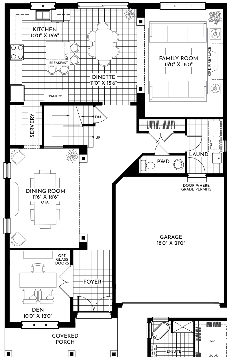
MAIN FLOOR ELEV. A
